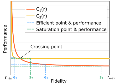
Figure 4. Illustration of efficient point and saturation point associated with learning curves.
